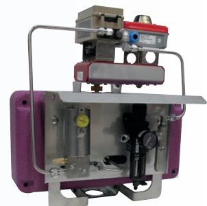
Remote Control Mode Smart positioner Communication Protocol ( HART, PROFIBUS, etc.).
